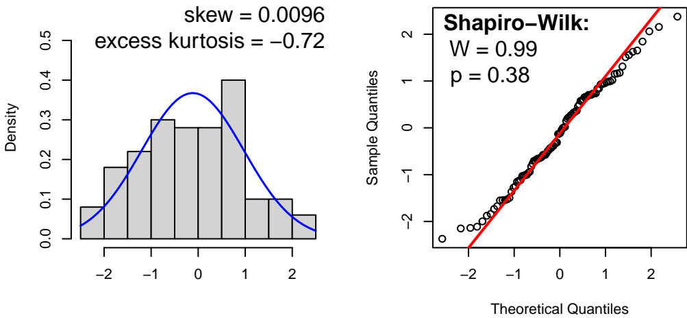
Population: exponential
