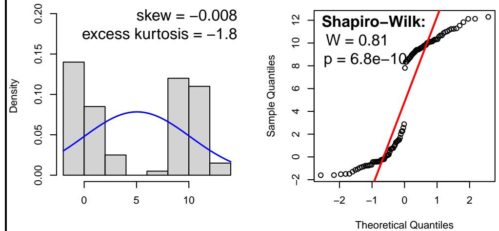
Population: bimodal
