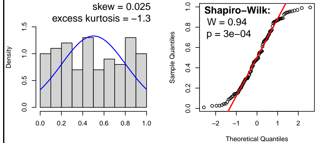
Population: bimodal
